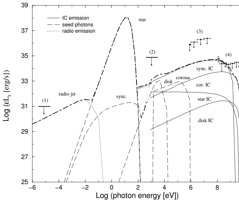
Fig. 2 The same as in Fig. 1 but for the source 3EG J1735+1500.
